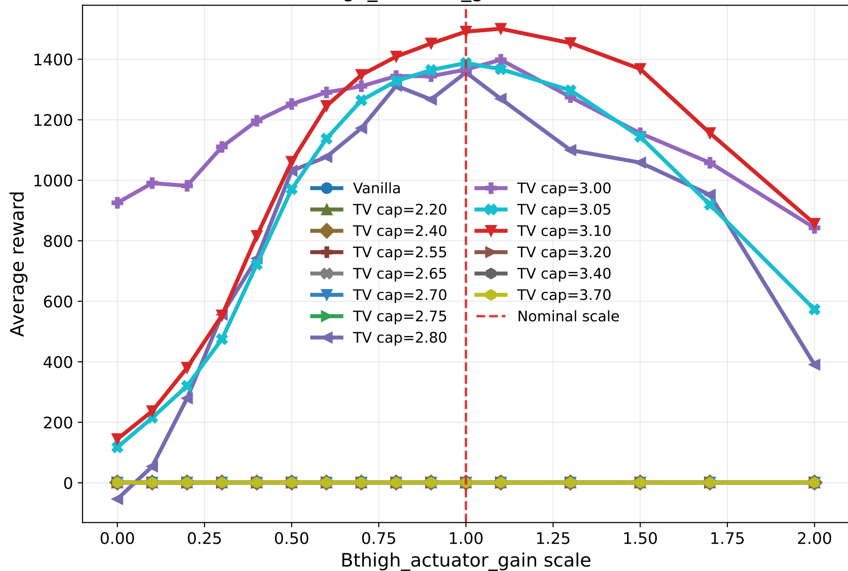
Bthigh_actuator_gain robustness
